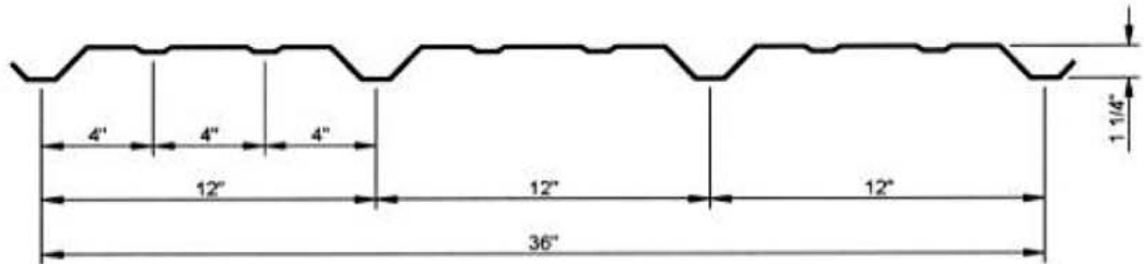
Panel Detail
